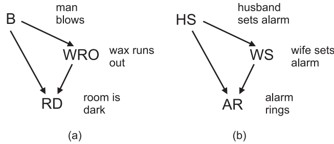
FIGURE 2. (a) Structural causal model for the Candle scenario. B = 1 ; WRO = \neg B ; RD = B \vee WRO . (b) Structural causal model for the Alarm scenario. HS = 1 ; WS = \neg HS ; AR = HS \vee WS . All variables are endogenous and propositional. Notice that although these models are isomorphic, we would desire them to yield different answers for certain causal queries.
