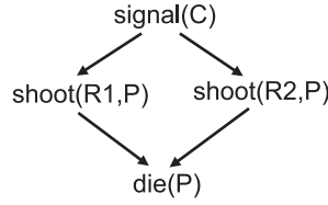
FIGURE 6. DAG representing time dependencies between actions in the Firing Squad scenario.
