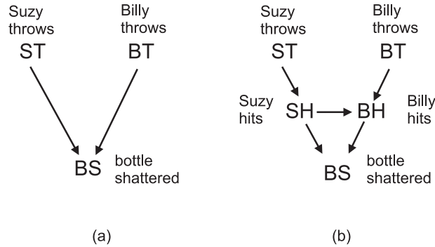
FIGURE 3. Structural causal models for the Bottle scenario. (a) ST=1 ; BT=1 ; BS = ST \vee BT . (b) ST=1 ; BT=1 ; SH=ST ; BH = BT \wedge \neg SH ; BS = SH \vee BH . All variables are endogenous and propositional.
