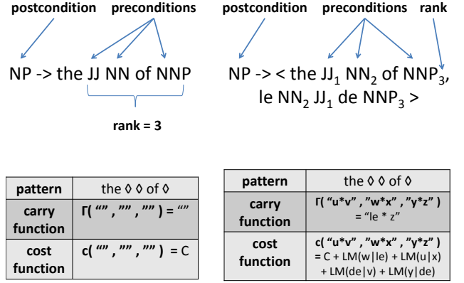
Figure 6: Deconstruction of a CFG rule (left) and SCFG rule (right) according to the definition of rule in Section 3.1. The carry function of the SCFG rule computes boundary words for a 2-gram language model. In the cost functions, C is a real number and \text{LM} returns the negative log of a language model query.
