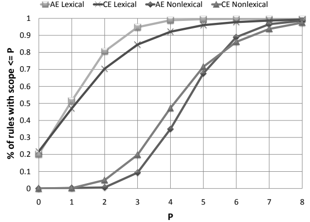
Figure 10: Breakdown of rules by scope (average per sentence in our test sets). In practice, most of the lexical rules applicable to a given sentence (95% for Arabic-English and 85% for Chinese-English) are scope 3 or less.
