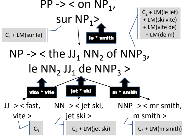
Figure 5: The cost of the SCFG derivation in Figure 3 (with an integrated language model score) can also be distributed to the nodes of the derivation, but to perform the local computations, information must be passed up the tree. We refer to this extra information as a carry .
